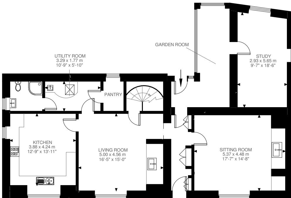
Ground Floor 1381 ft 2
